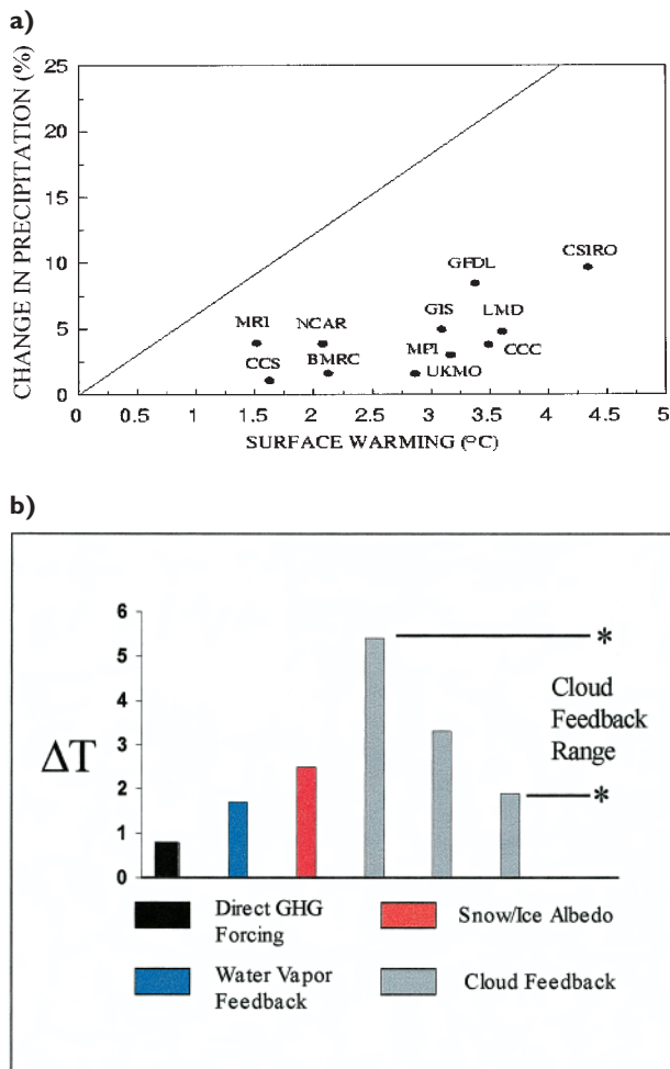
FIG. 2. (a) The responses of various coupled ocean-atmosphere GCMs to an imposed doubling of \text{CO}_2 . The different models can be identified according to the indicated organization. (b) The response of a single climate model to an imposed doubling of \text{CO}_2 as different feedbacks are systematically added in the model (starting from left to right and adapted from Senior and Mitchell 1993). Different treatments of cloud processes in the model produce a large spread in predicted surface temperature due to \text{CO}_2 doubling.
