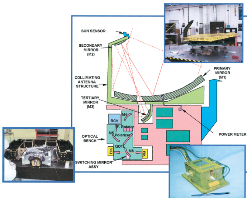
FIG. 8. The radar is composed of the following subsystems: the RFES, the HPA, the antenna subsystem, and the digital subsystem. Shown is a schematic of the antenna and HPA subsystems. The inset figures are actual photographs of flight hardware. The antenna subsystem consists of (top inset) the antenna, and quasi-optical transmission line built on an optical bench (left inset). (lower right inset) EIK, a key component of the HPA, which is required to amplify the transmitted pulse to 1.7 kW. The approximate 2-kW output of the flight model EIK exceeds this requirement.
