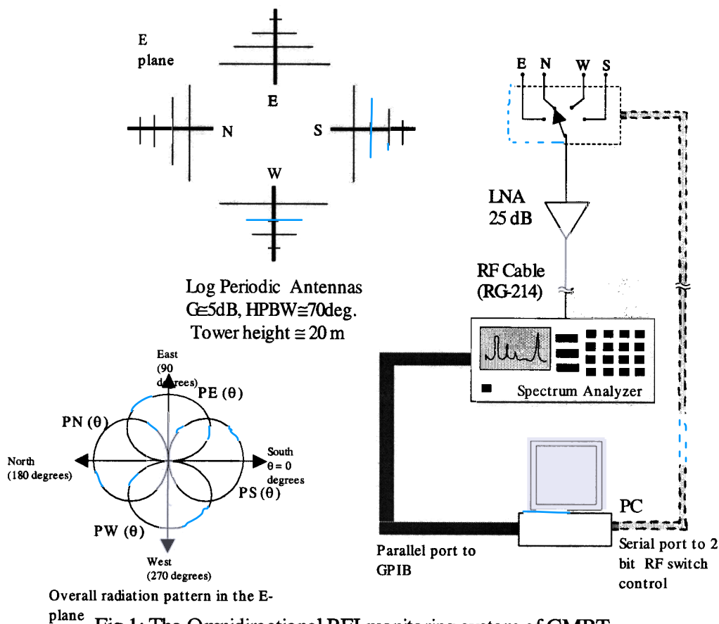
Fig. 1: The Omnidirectional RFI monitoring system of GMRT
